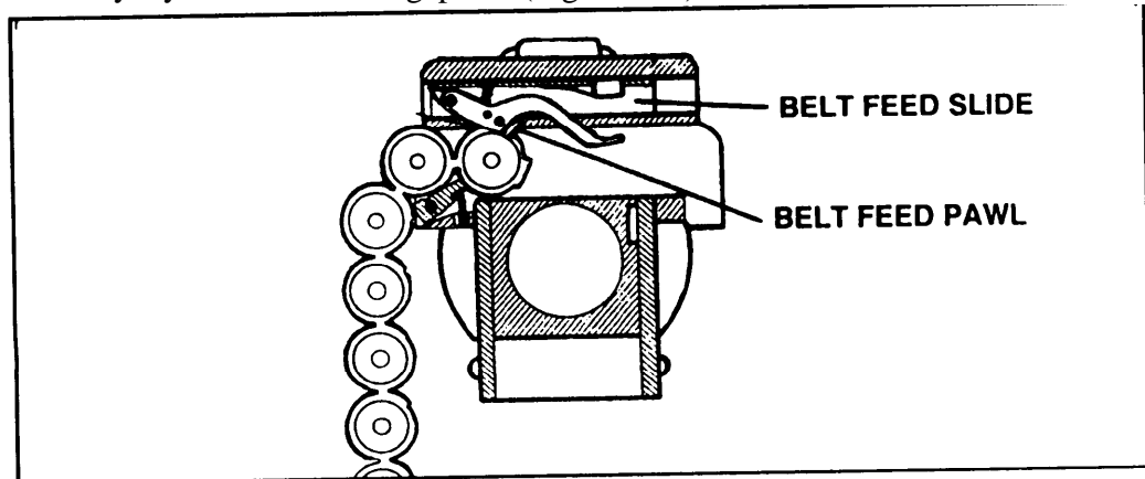
Figure 3-5. Feeding – step 1.
